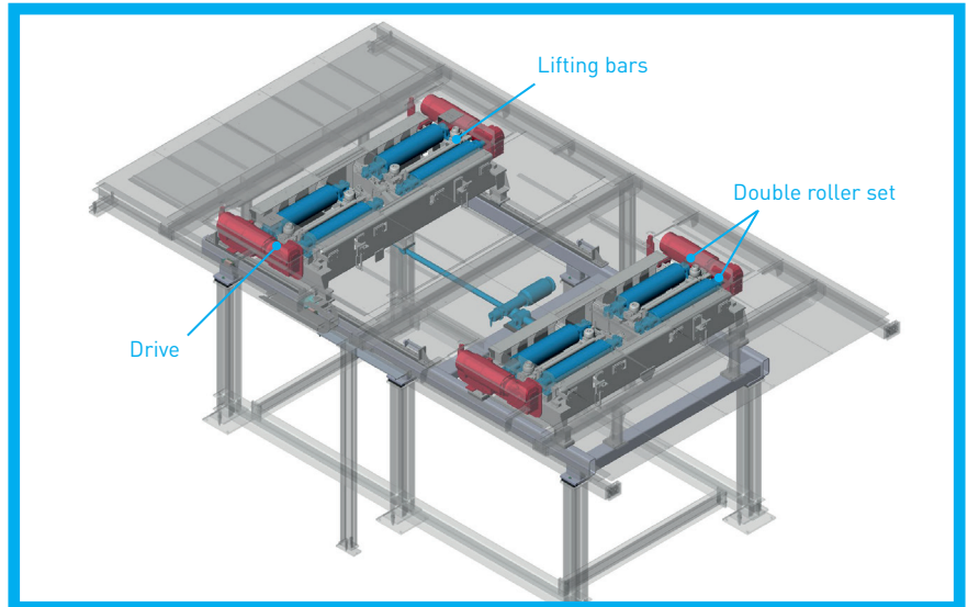
Layout x-brake
